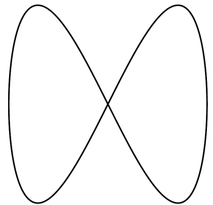
i / The Lissajous figure x = \cos t , y = \sin 2t .
